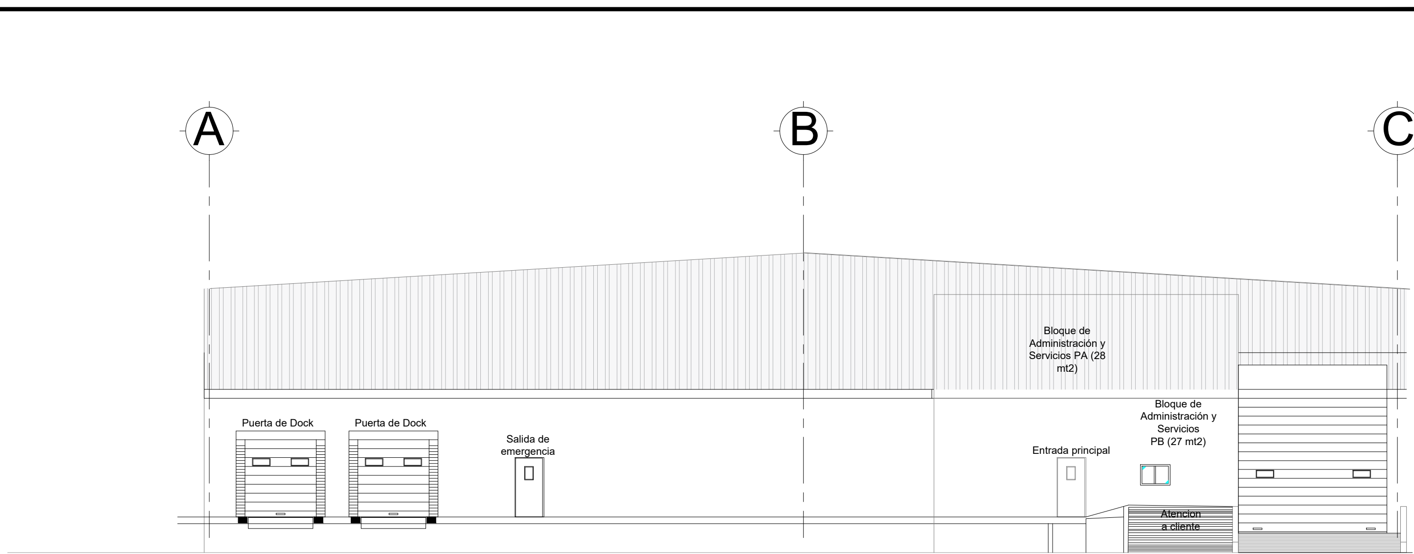
FACHADA PRINCIPAL
